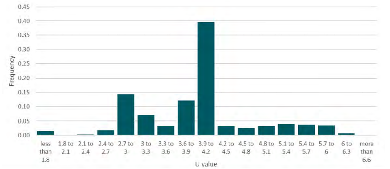
Figure 10: Distribution of U values for windows (Source: Document F)
